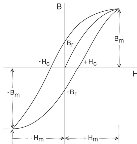
Figure 3 - Hysteresis
