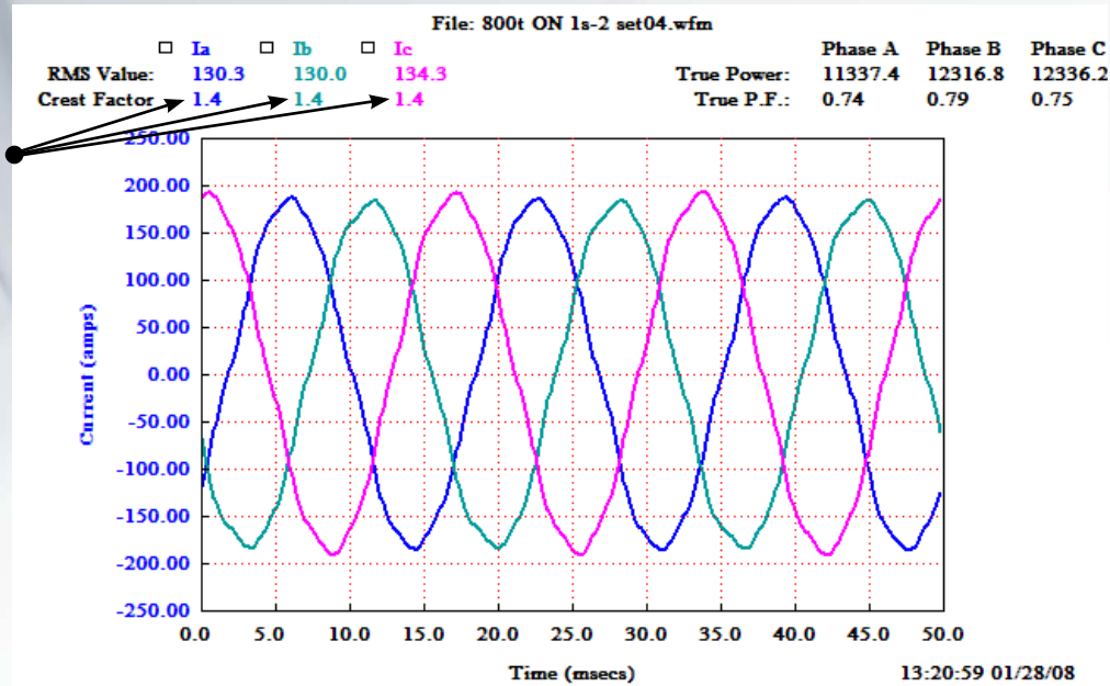
Figure 5. Current distribution on a three phase motor 3 months after EP
